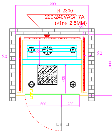
Plane graph
